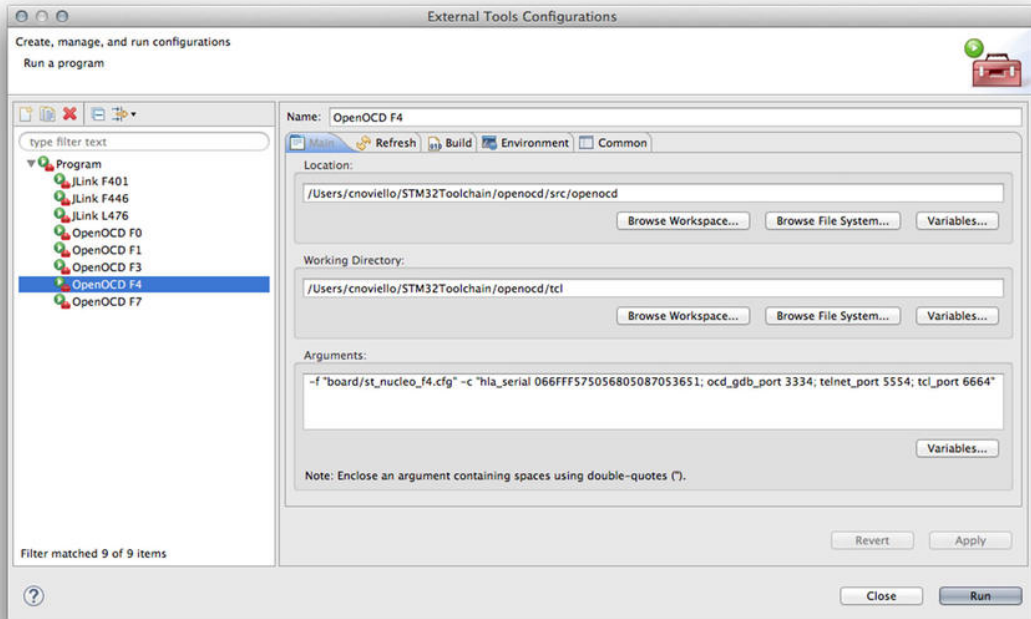
Figure 26: How to fill the External Tools Configurations fields when using two ST-LINK simultaneously
