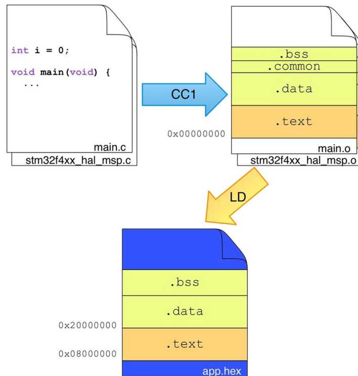
Figure 2: The compilation process from the source file to the final binary image
