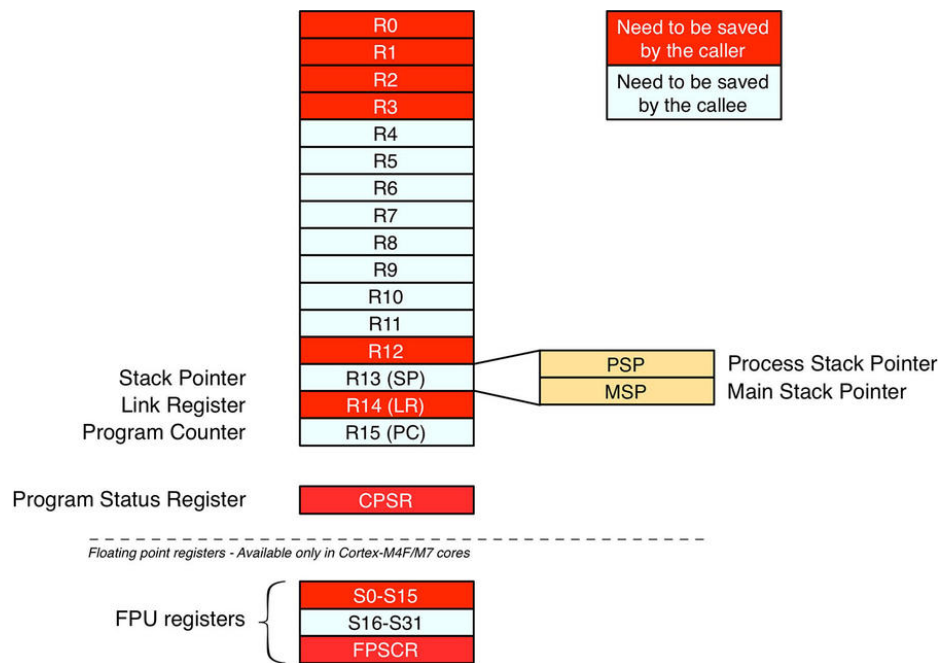
Figure 1: Cortex-M CPU core registers
