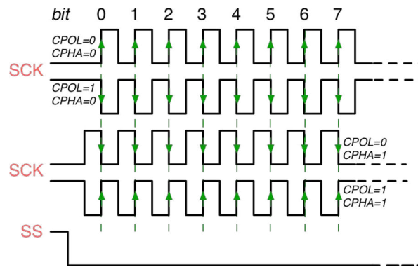
Figure 4: The SPI timing diagram according to CPOL and CPHA settings
