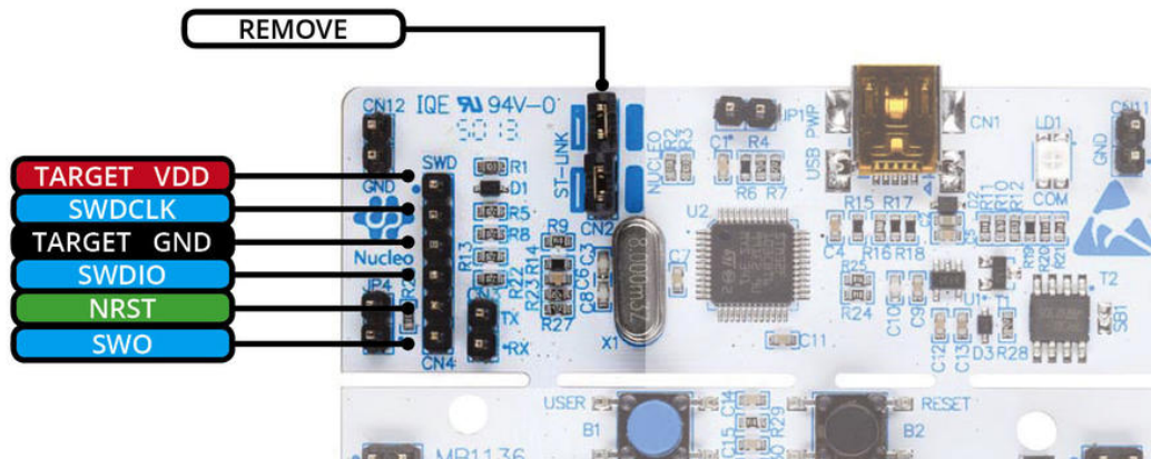
Figure 5: How to use the Nucleo as ST-LINK debugger
