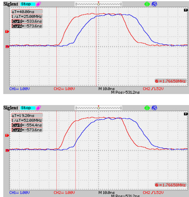
Figure 8: The top figure shows the slew rate of PC4 pin and the one below the slew rate of PC8 pin
