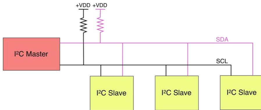
Figure 1: A graphical representation of the I 2 C bus
