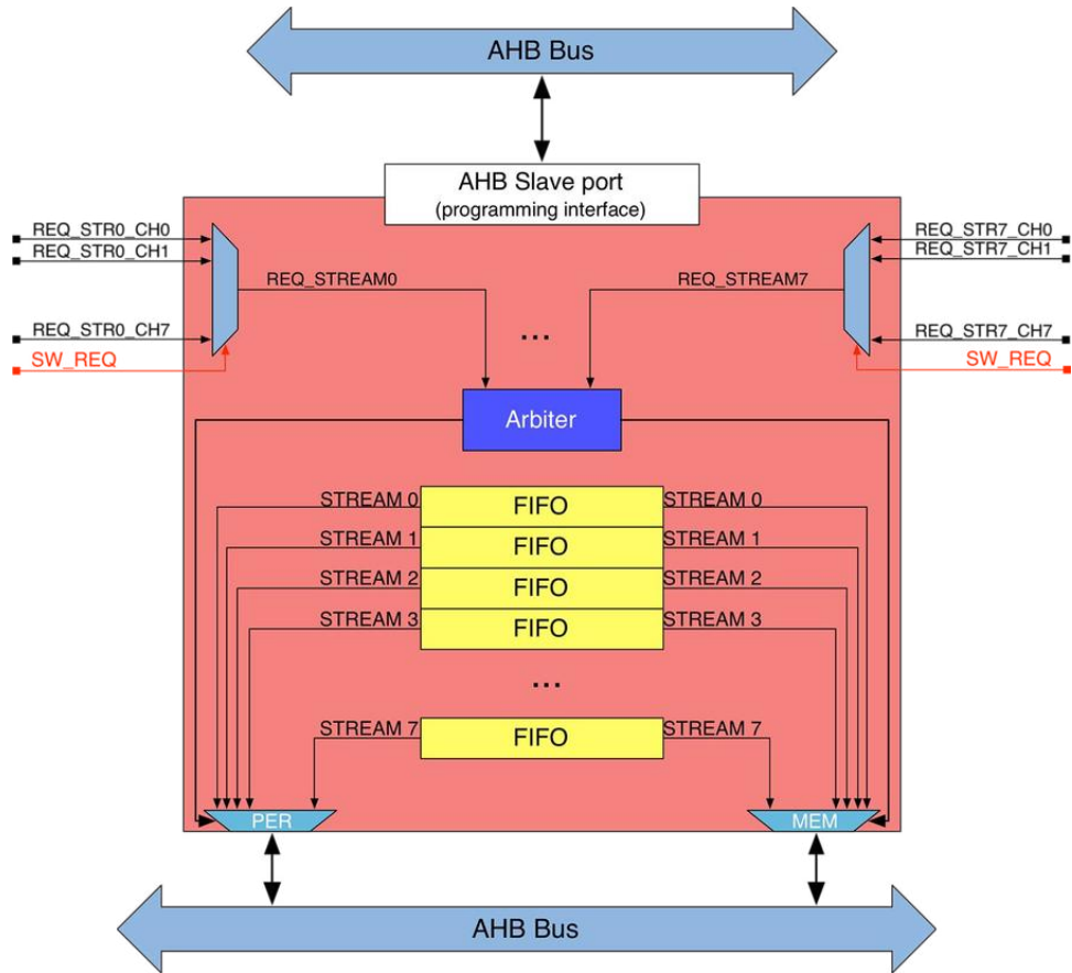
Figure 5: The DMA architecture in an STM32F2/F4/F7 MCU
