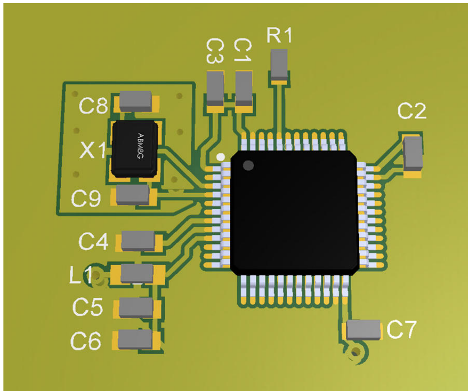
Figure 4: A good design way to place external crystals using a separated ground plane
