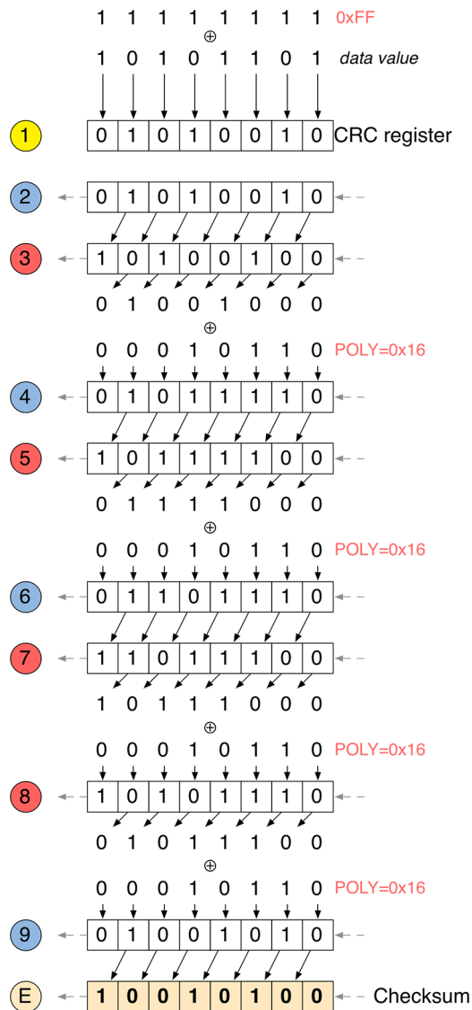
Figure 1: How CRC checksum is computed in an STM32
