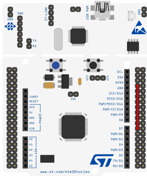
Figure 12: How to connect the TI2FP2 pin to AVDD pin in a Nucleo-F030R8 board
