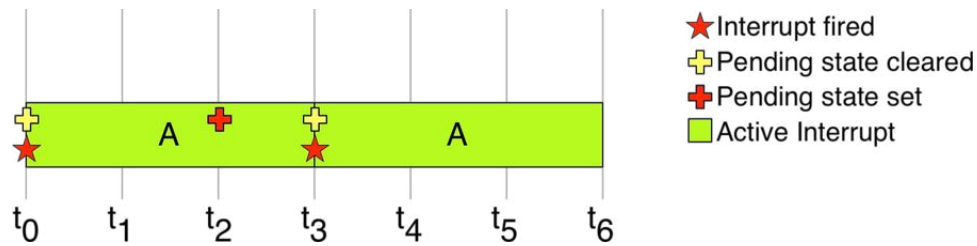
Figure 9: How an interrupt can be forced to fire again setting its pending bit
