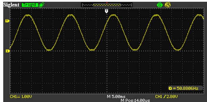
Figure 3: The output sine wave generated with the DAC peripheral
