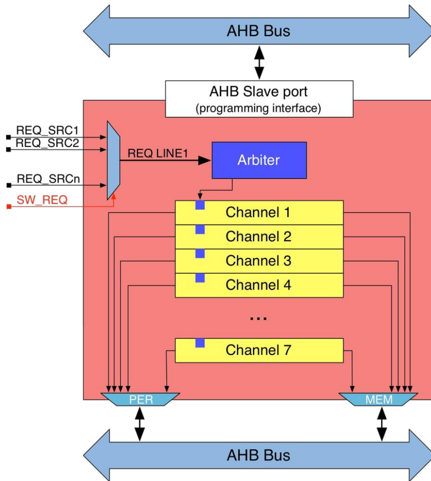
Figure 3: A representation of the DMA structure (other request lines omitted)
