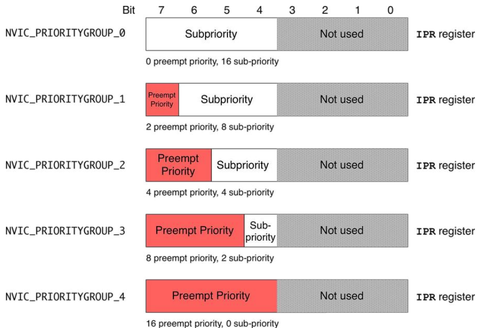
Figure 18: The subdivision of IPR bits between preemption priority and sub-priority
