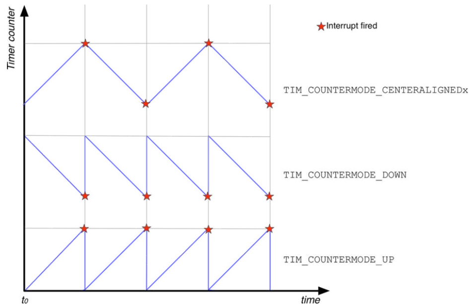
Figure 15: The three major counting modes of a general purpose timer
