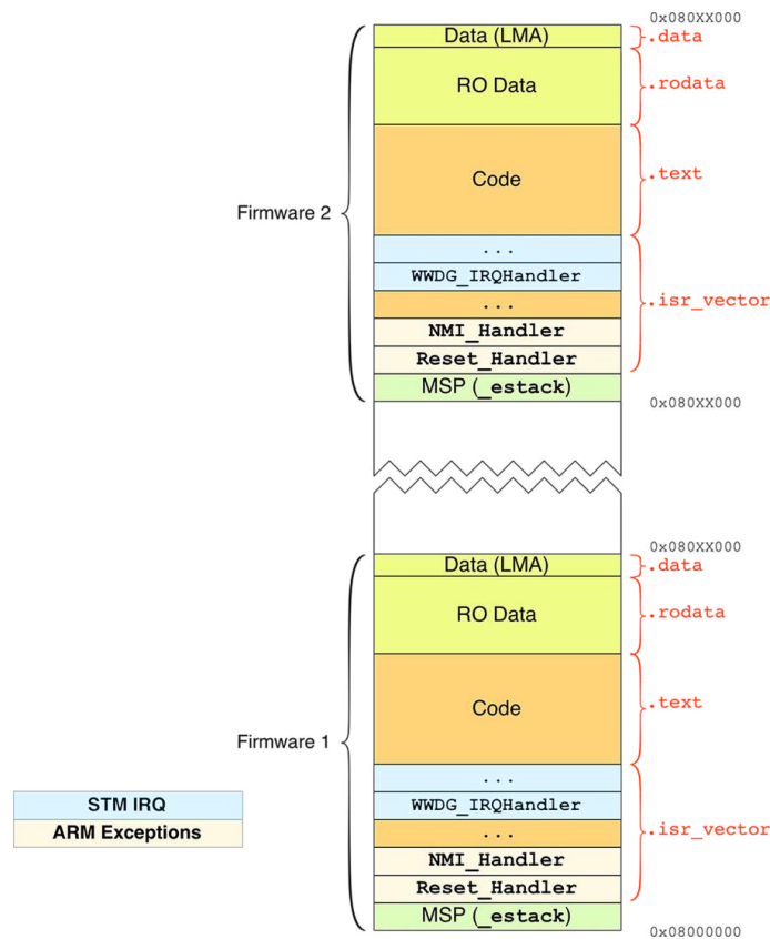
Figure 1: Two independent firmware images may be stored inside the flash memory
