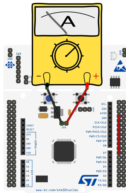
Figure 5: How to measure the MCU power consumption in a Nucleo board
