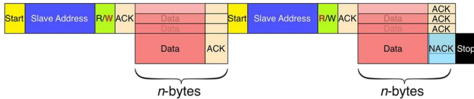
Figure 5: The structure of a combined transaction
