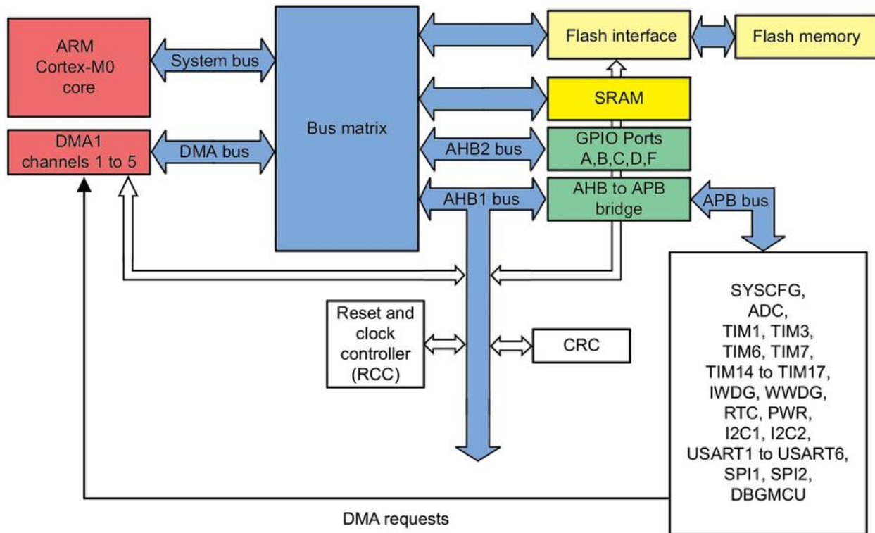
Figure 2: bus architecture of an STM32F030 microcontroller
