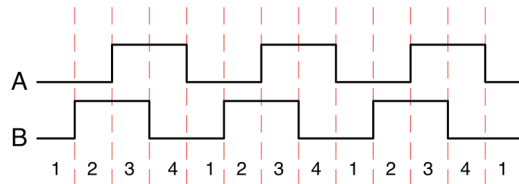
Figure 32: The square waves emitted by a quadrature encoder on A and B channels
