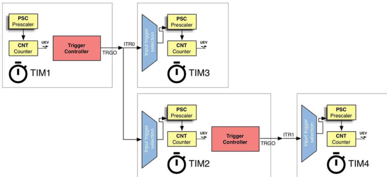
Figure 11: The combination of master/slave modes allows to configure timers in a hierarchical structure
