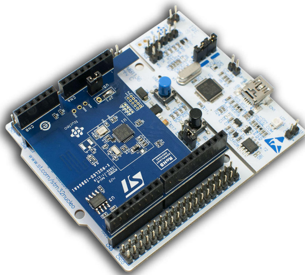
Figure 24: The BlueNRG expansion shield
