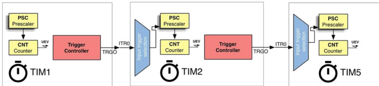
Figure 10: The combination of master/slave modes allows to configure timers in cascade
