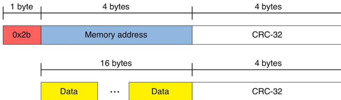
Figure 6: The structure of the CMD_WRITE
