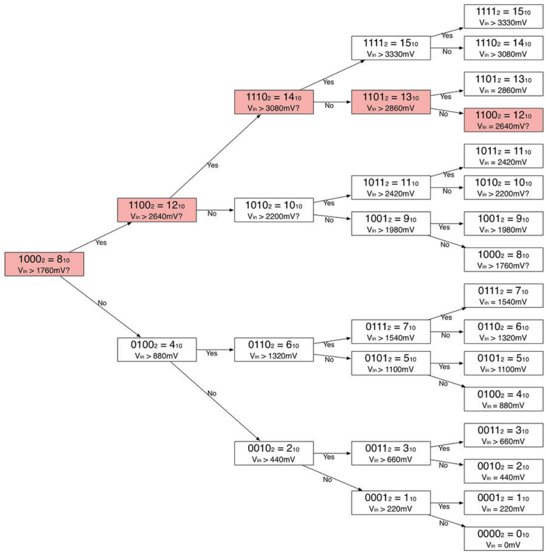
Figure 3: The conversion process made by a SAR ADC
