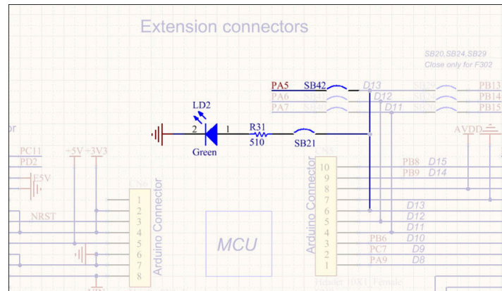
Figure 11: LD2 connection to PA5
