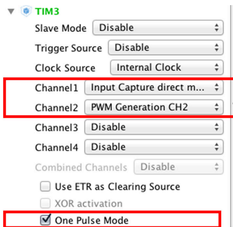
Figure 31: How to enable the One Pulse mode in a timer
