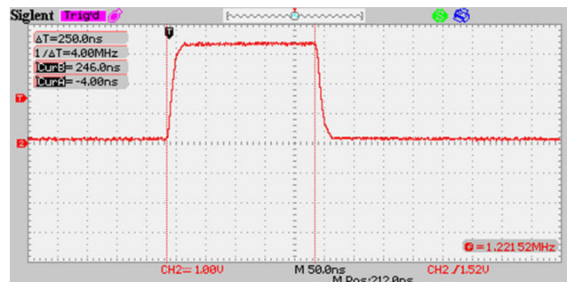
Figure 10: Switching frequency when toggling an I/O through bit-banding region
