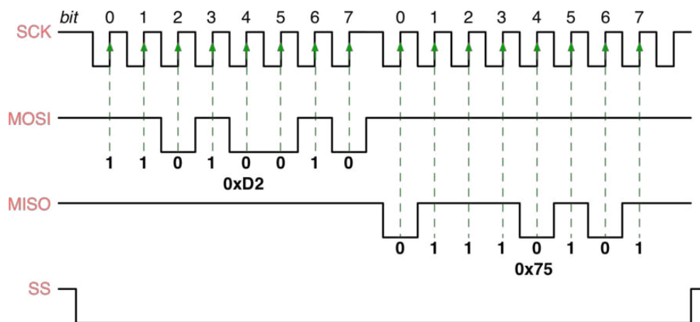
Figure 3: How data is exchanged over a SPI bus in a half-duplex transmission
