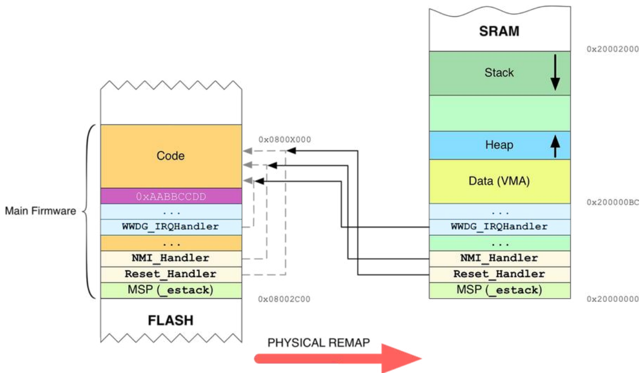
Figure 7: How the vector table can be relocated in STM32F0 microcontrollers
