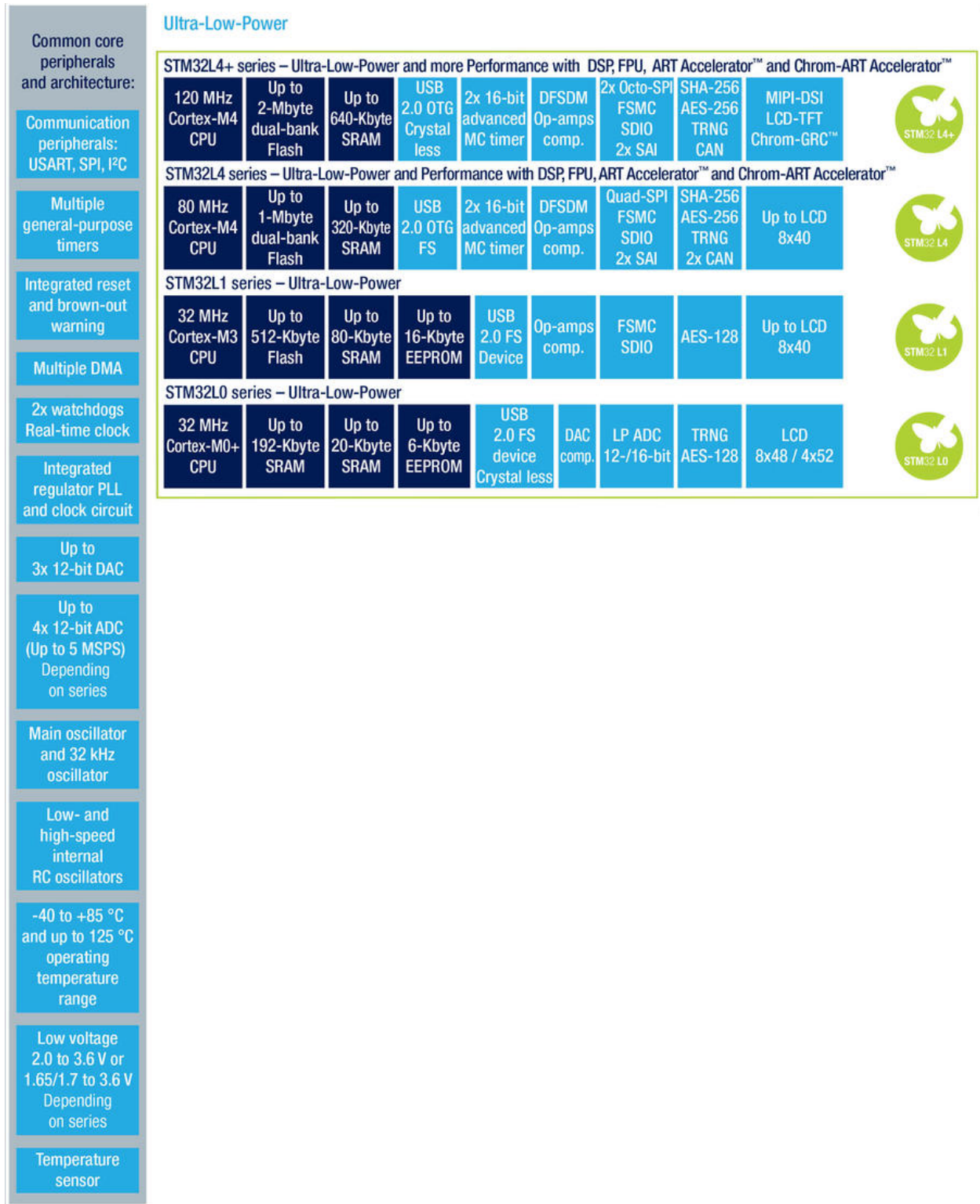
Figure 14: STM32 portfolio
