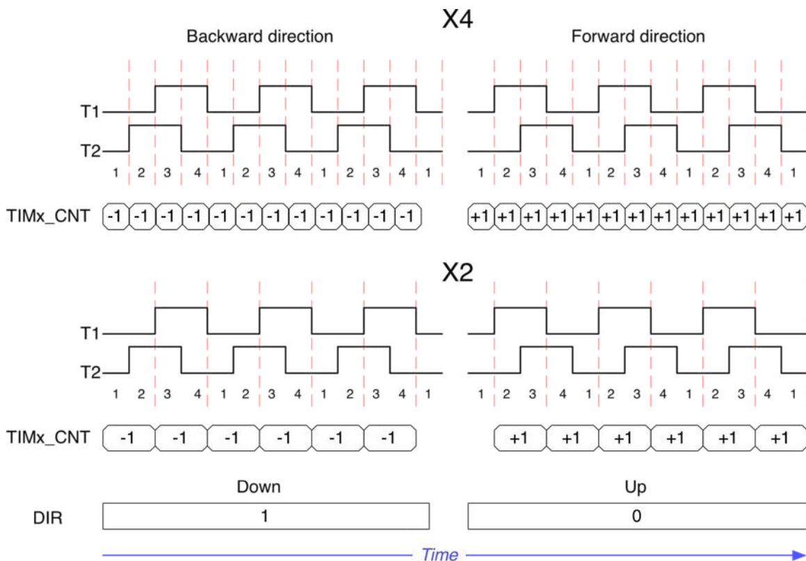
Figure 33: How encoder speed and direction are computed by a timer in encoder mode
