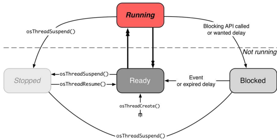
Figure 10: The possible states of a thread in FreeRTOS
