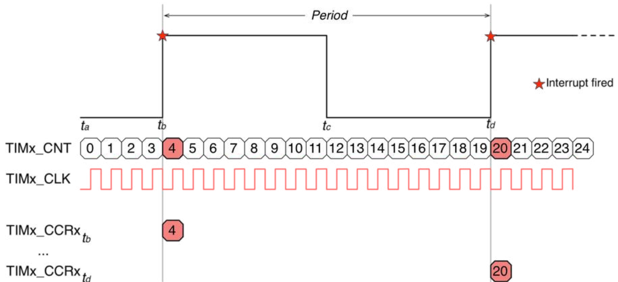
Figure 17: The capture process of an external signal feeding one of the timer channels
