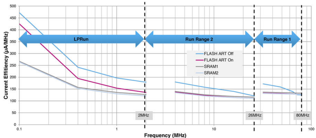
Figure 8: Power optimization vs frequency in STM32L4-series
