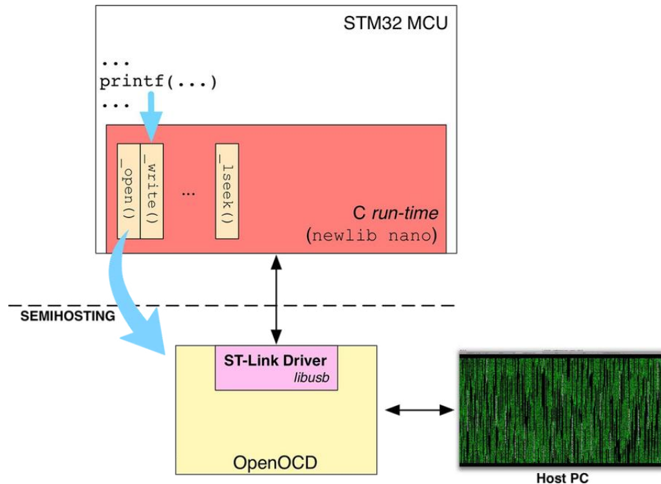
Figure 19: How syscalls are routed to debugger using semihosting
