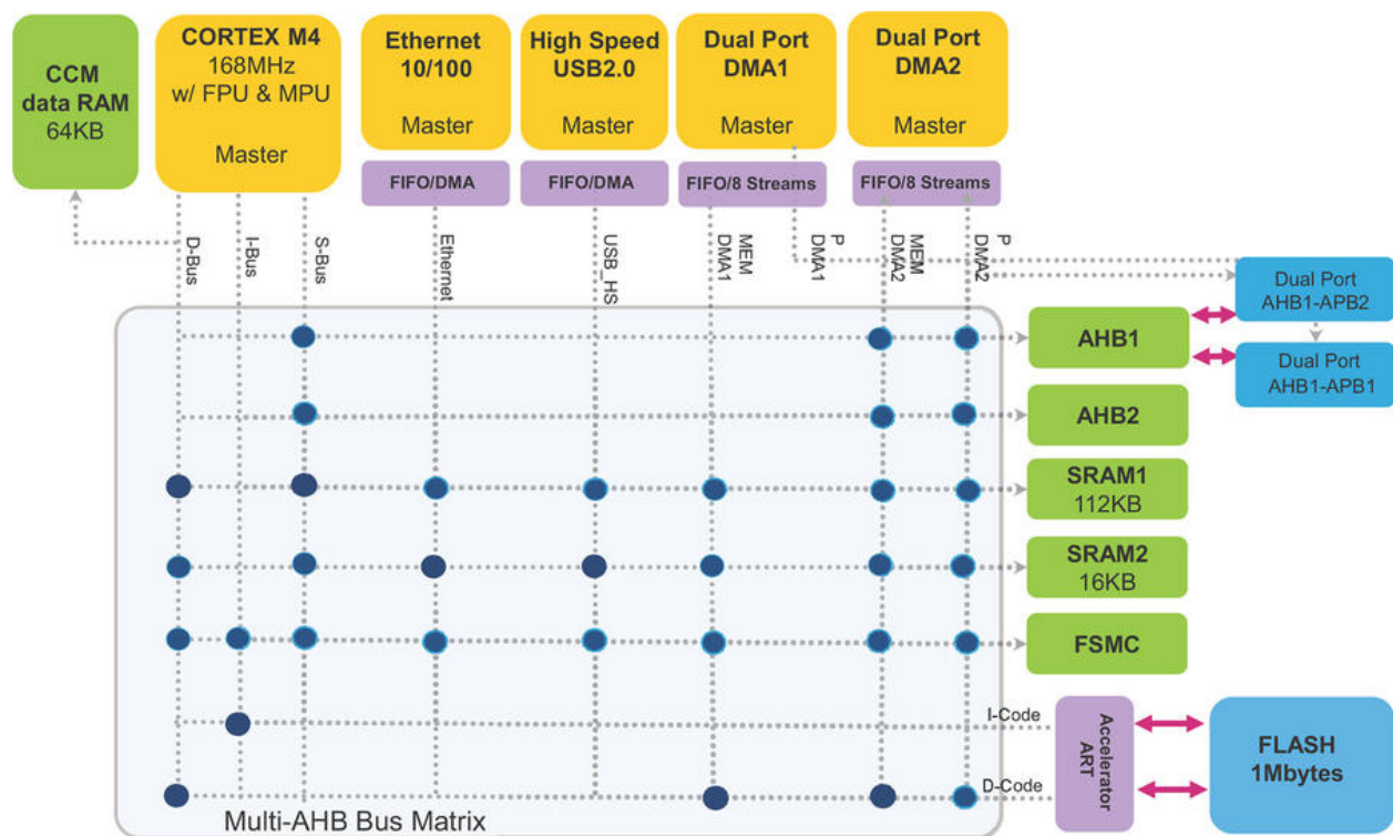
Figure 6: The multi-layer BusMatrix in an STM32F405 MCU
