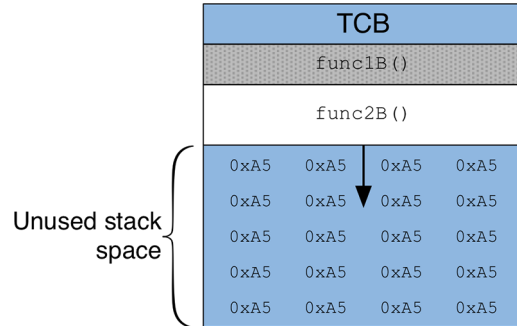
Figure 12: How FreeRTOS fills the stack with a fixed value (0xA5) to detect stack overflows
