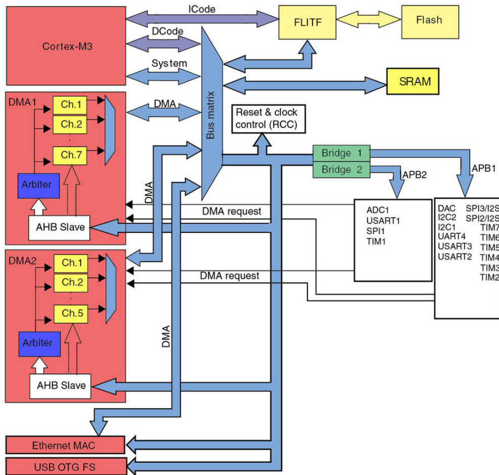
Figure 4: The bus architecture in an STM32F1 MCU from the Connectivity Line
