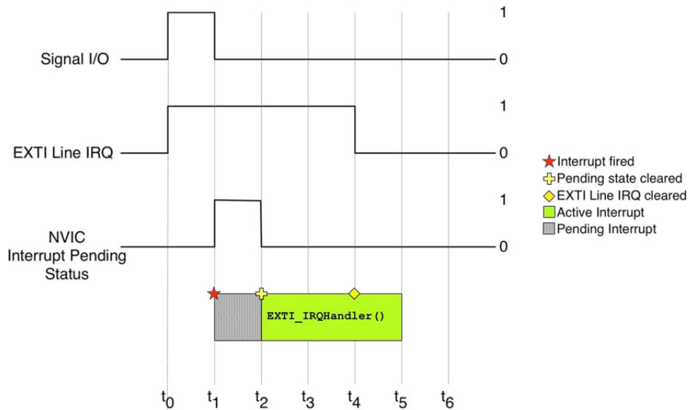
Figure 11: The relation between the peripheral IRQ and the corresponding interrupt
