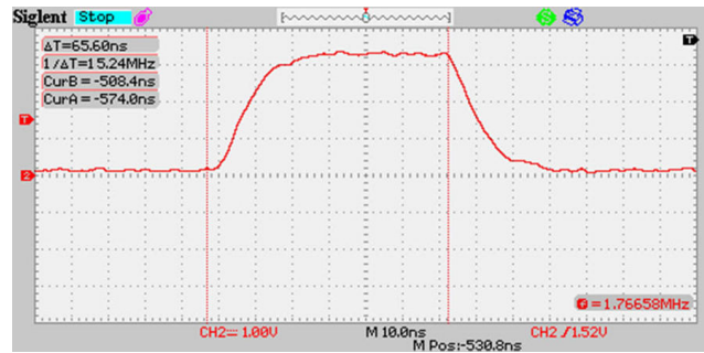
Figure 9: The maximum I/O switching frequency achieved with an STM32F446
