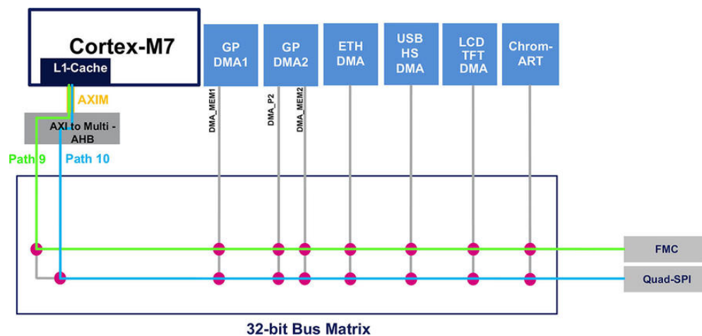
Figure 6: FMC and QuadSPI external memory controllers
