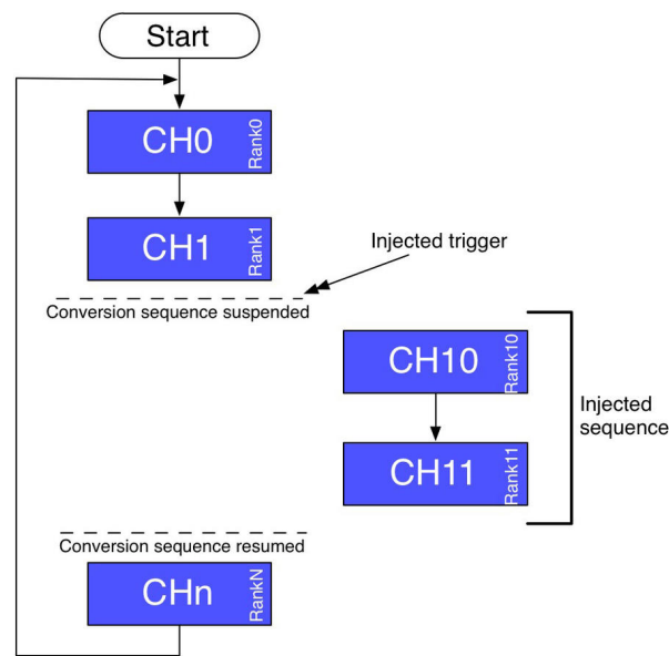
Figure 9: Injected conversion mode
