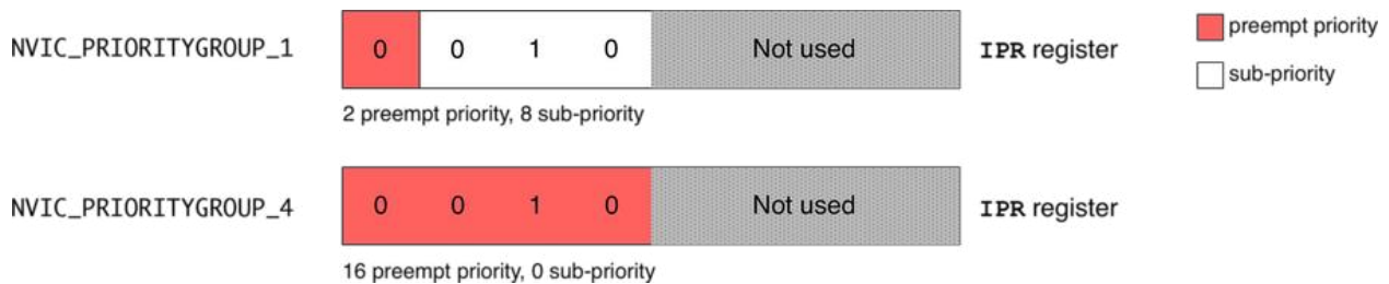
Figure 20: What happens to the C ISR priority when the priority grouping is lowered from 4 to 1
