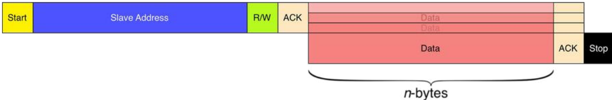
Figure 4: A transmission in burst mode where multiple bytes are exchanged in one transaction
