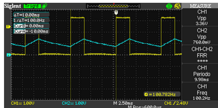
Figure 25: The effect of a low-pass filter with cut-off frequency equal to 15.9Hz
