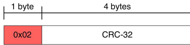
Figure 4: The structure of the CMD_GETID
