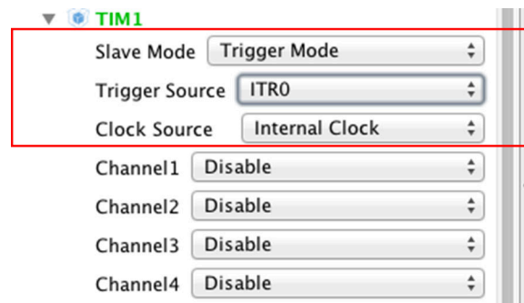
Figure 13: How to configure a timer in slave mode
