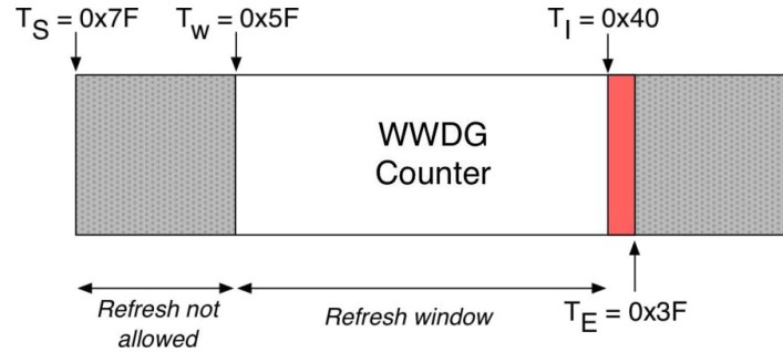
Figure 2: How the temporal window defines the counter interval within which it is allowed to refresh the WWDG timer
