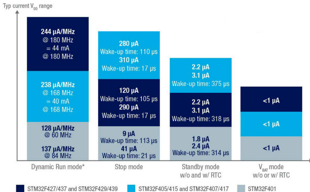
Figure 4: The power consumption of some STM32F4 MCU
