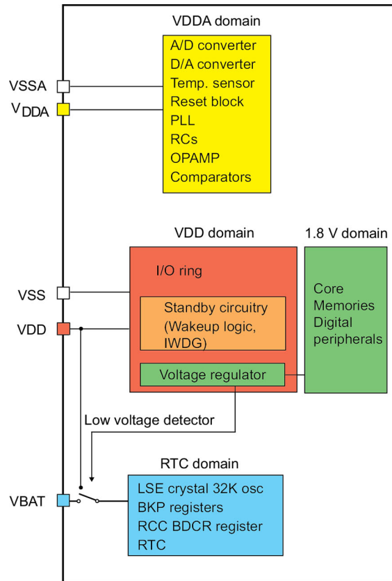
Figure 3: The power sources in an STM32F microcontroller
