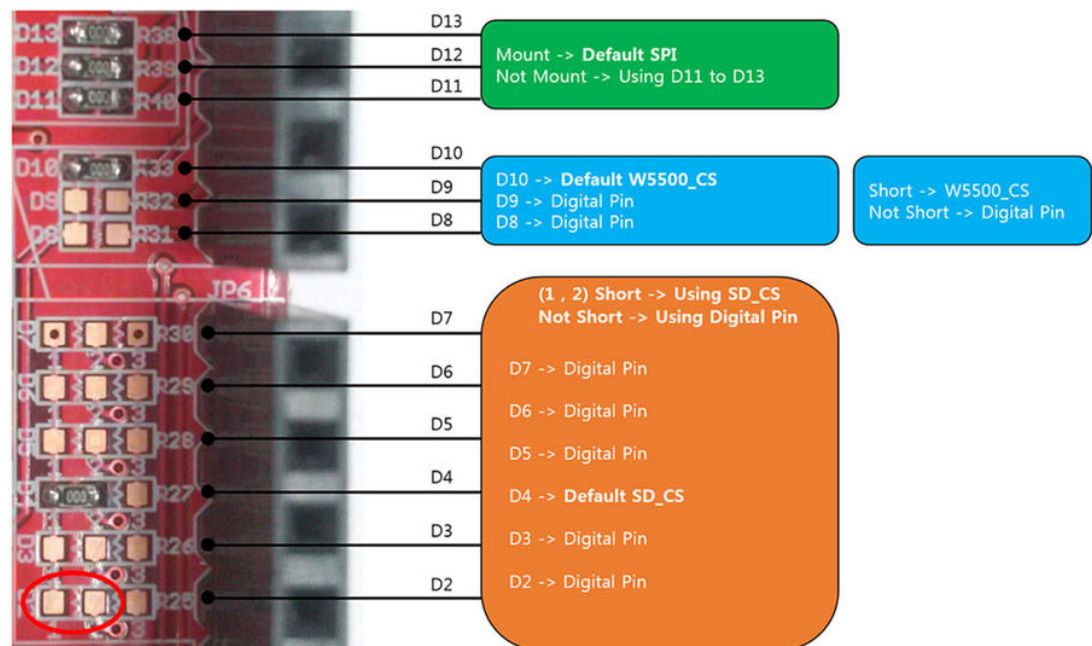
Figure 6: To enable INTn pin, it is required to short 1-2 pads
