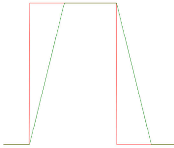
Figure 7: Slew rate effect on a square wave - red=desired output, green=actual output
