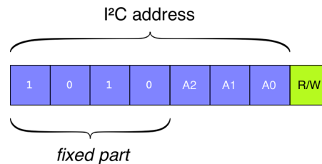
Figure 7: How the 24LCxx I 2 C address is composed.
