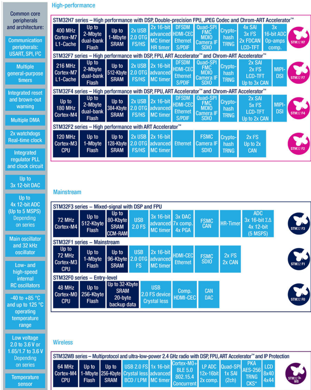
Figure 13: STM32 portfolio
