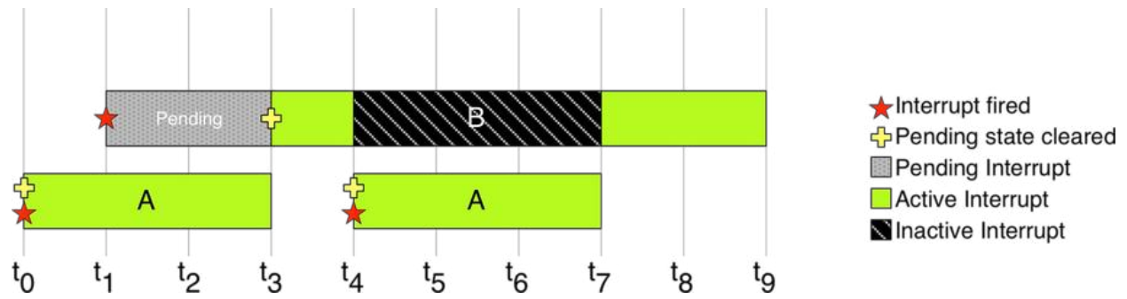
Figure 8: The relation between the active status and interrupts priority
