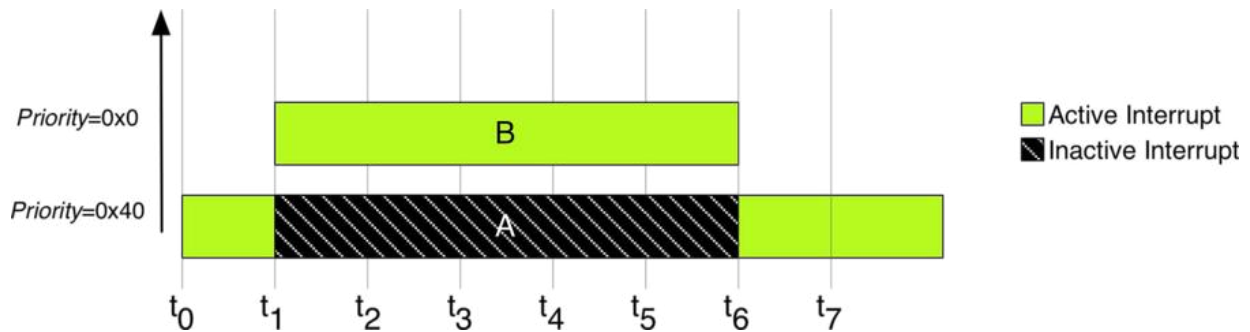
Figure 14: Preemption of interrupts in case of concurrent execution
