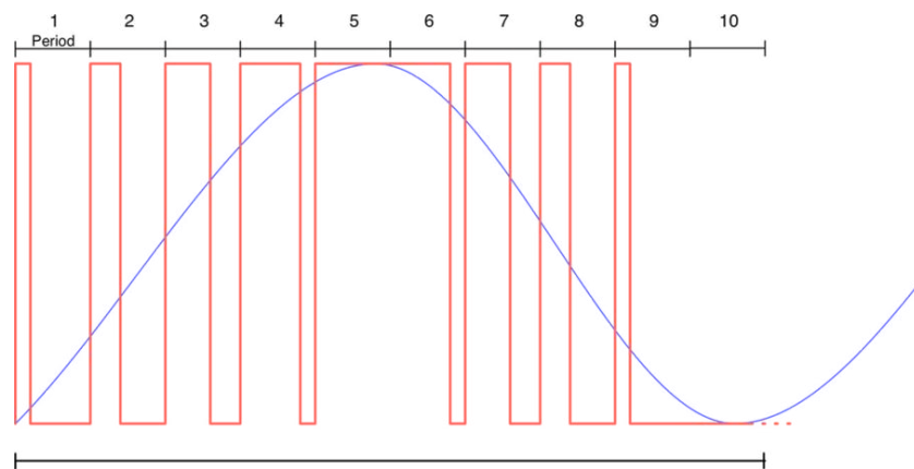
Figure 27: How a sine wave can be approximated with multiple PWM signals
