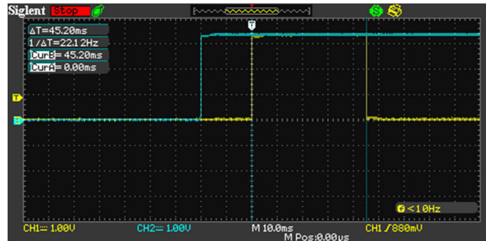
Figure 30: How the One Pulse mode works
