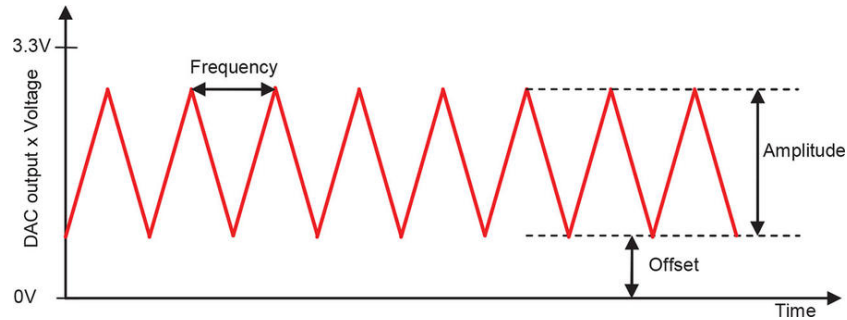
Figure 4: A triangular wave generated with the DAC
