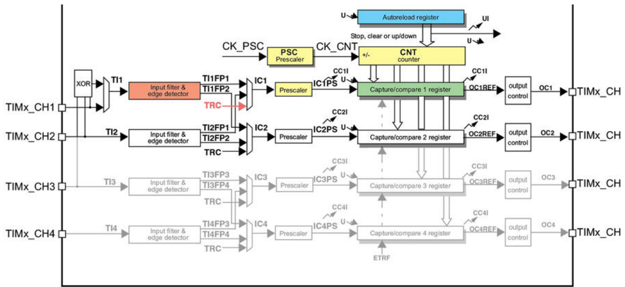
Figure 16: The structure of the input channel in a general purpose timer
