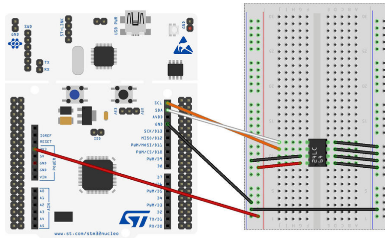
Figure 8: How to connect a Nucleo to a 24LCxx EEPROM
