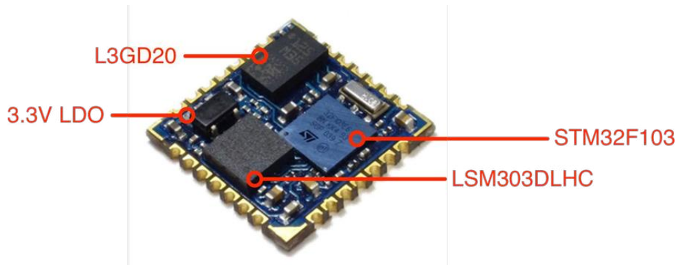
Figure 11: The INEMO-M1 module by ST
