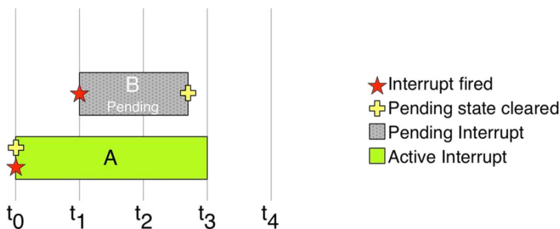
Figure 10: IRQ servicing can be canceled clearing its pending bit before it is executed
