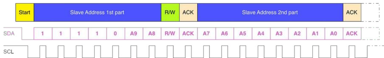
Figure 3: The message structure in case if 10-bit addressing is used
