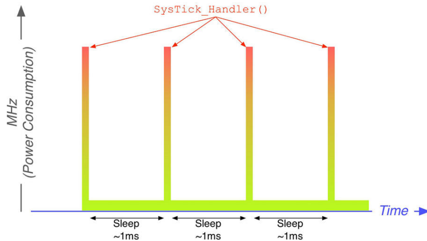
Figure 15: The effects of SysTick interrupts on the power consumption
