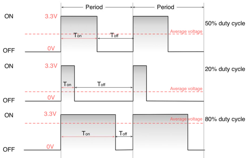
Figure 23: Three different duty cycles - 50%, 20% and 80%
