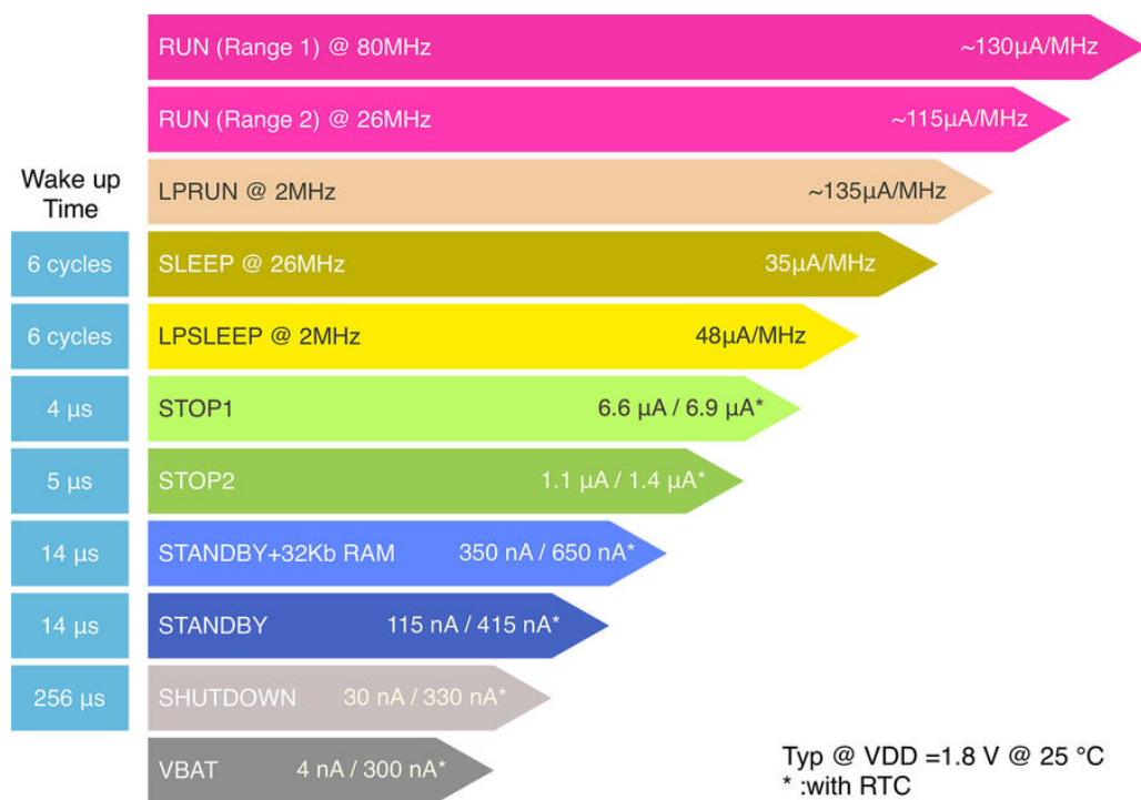
Figure 7: The eleven power modes supported by STM32L4 microcontrollers
