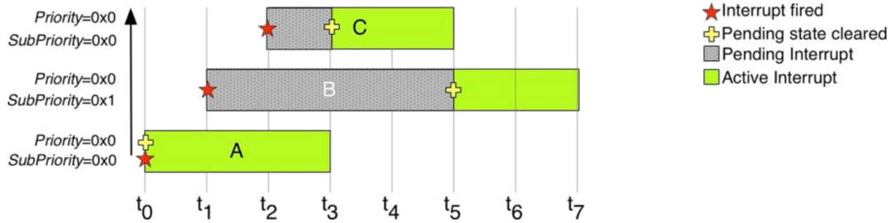
Figure 17: If two interrupts with the same priority are pending, the one with the higher sub-priority is executed first
