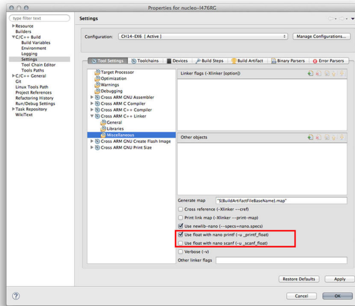
Figure 13: How to enable float support in printf() and scanf()
