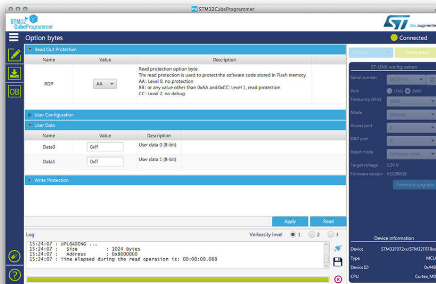
Figure 1: The Option Bytes configuration dialog in the STM32CubeProgrammer
