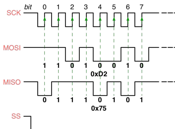
Figure 2: How data is exchanged over a SPI bus in a full-duplex transmission
