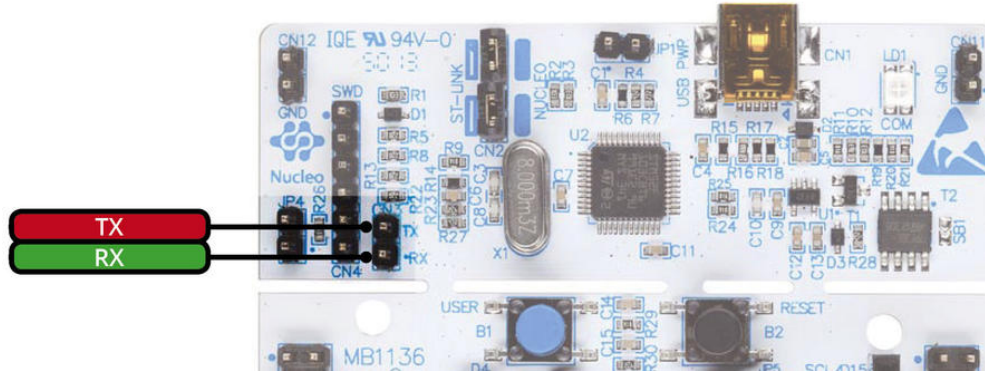
Figure 6: The CN3 connector allow to use the ST-LINK VCP with any other USART
