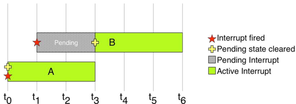
Figure 7: The relation between the pending bit and the interrupt active status
