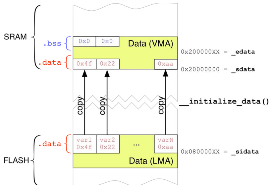
Figure 3: The copy process of initialized data from the flash to the SRAM memory
