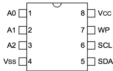
Figure 6: The pinout of a 24LCxx EEPROM with a PDIP-8 package
