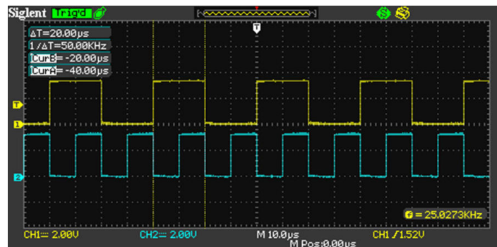
Figure 22: Channel 2 is configured to switch twice as fast as channel 1
