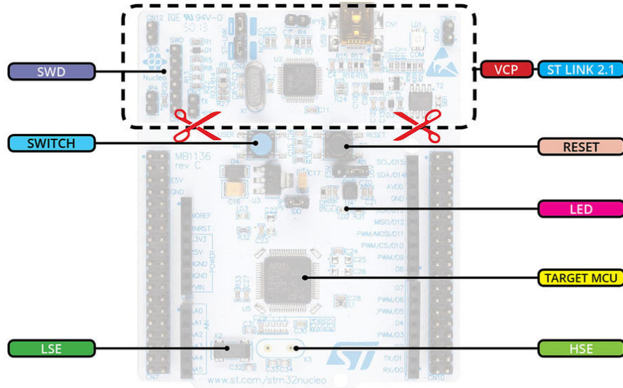
Figure 21: The relevant parts of a Nucleo board
