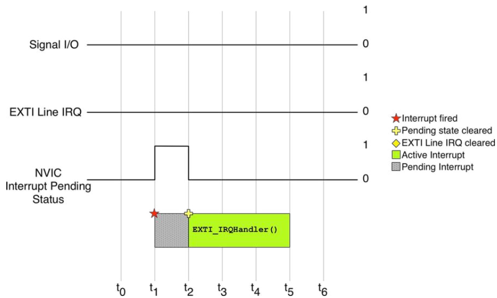
Figure 12: When an interrupt is forced setting its pending bit, the corresponding peripheral IRQ remains unset
