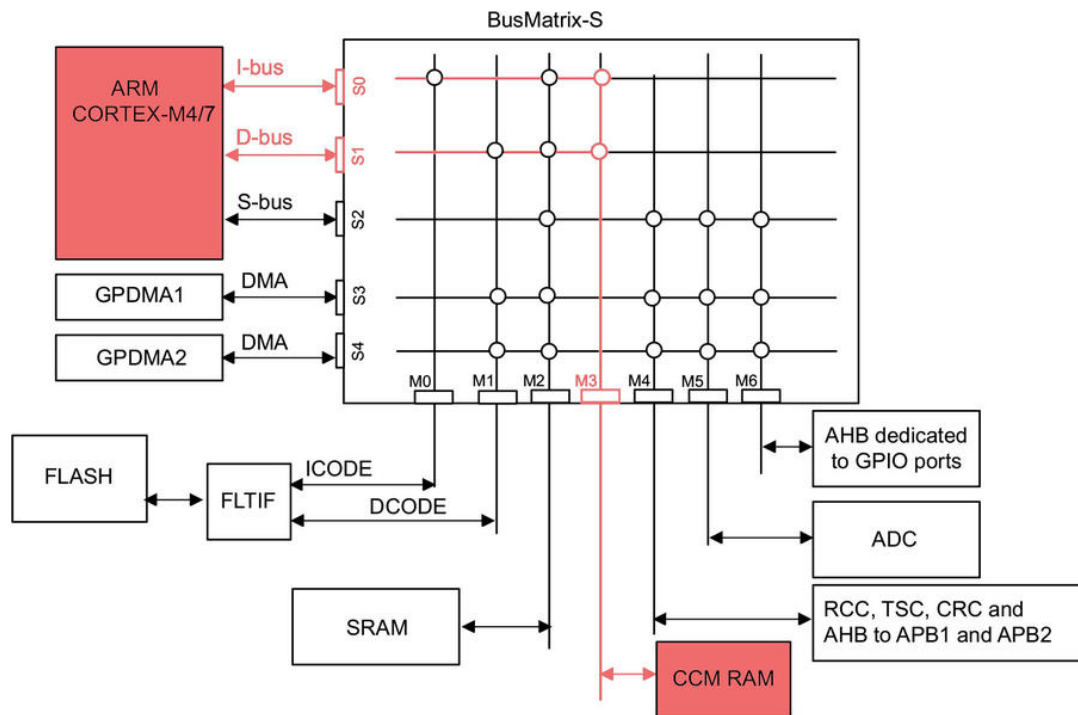
Figure 5: The direct connection between the Cortex-M core and the CCM SRAM
