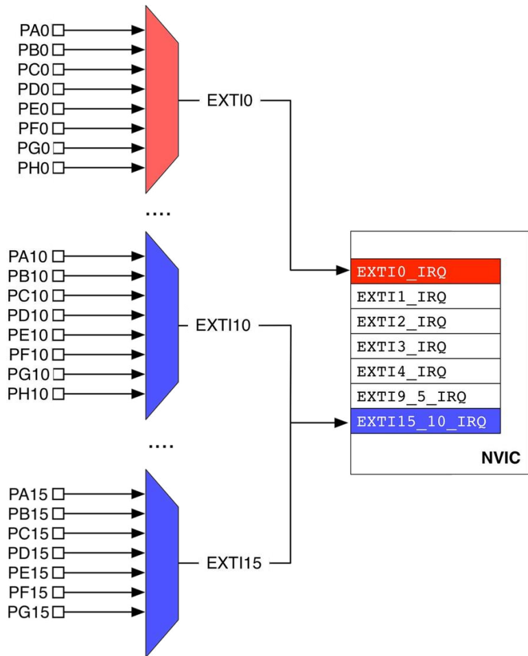
Figure 3: The relation between GPIO, EXTI lines and corresponding ISR in an STM32F4 MCU
