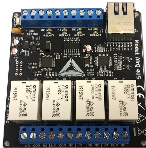
Figure 2: A custom device made with an STM32F0 MCU (on the left) and a W5500 IC (on the right)
