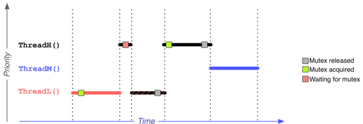
Figure 14: How the priority inversion problem is addressed by temporary increasing the priority of ThreadL
