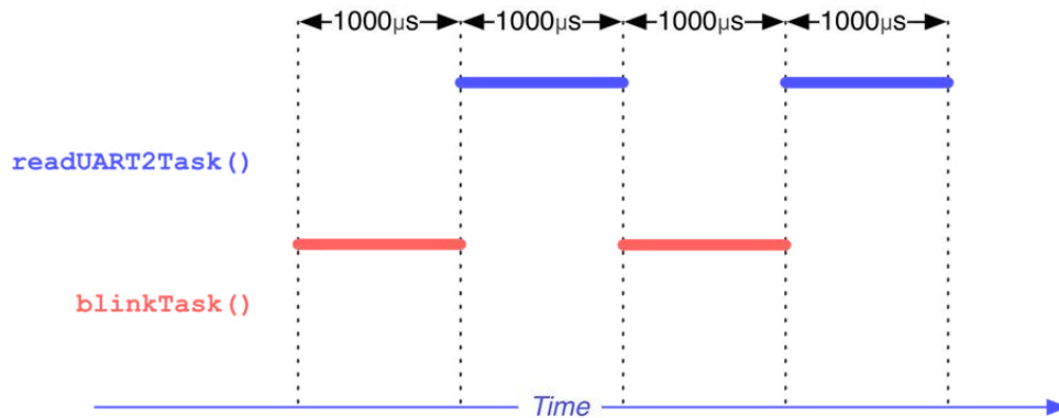
Figure 1: How an OS schedules the tasks execution by assigning them a fixed quantum time
