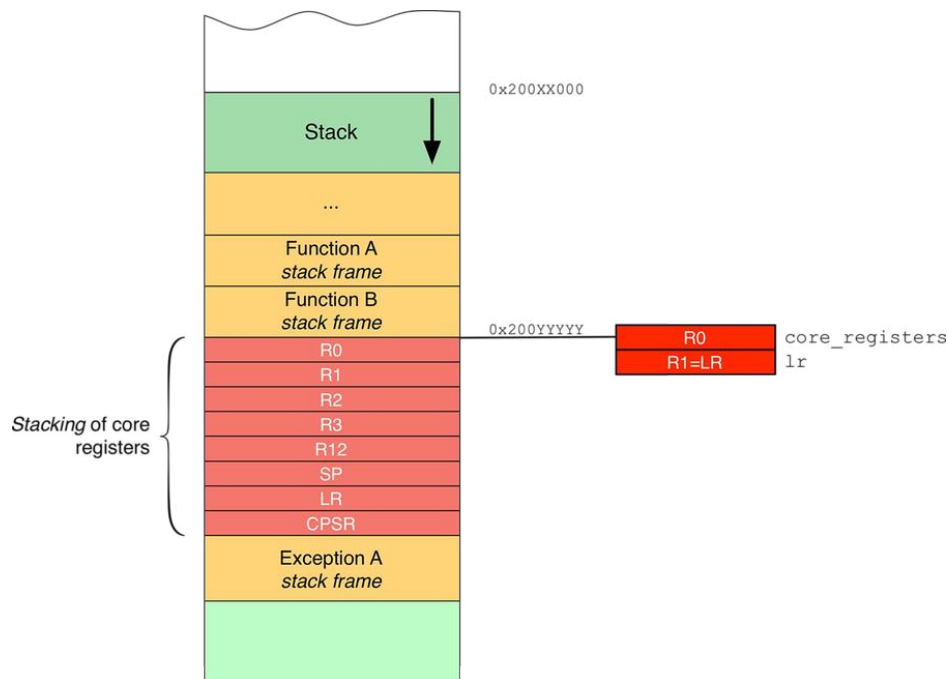
Figure 3: How current R0-R1 registers point to stacked register and actual LR register
