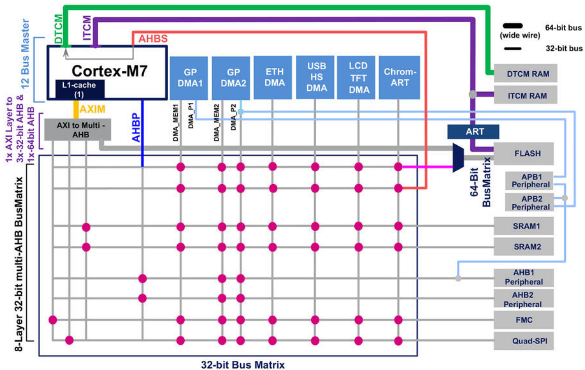
Figure 4: The bus matrix in an STM32F7 MCU
