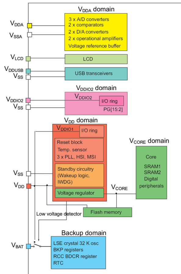
Figure 6: The power sources in an STM32L4 microcontroller
