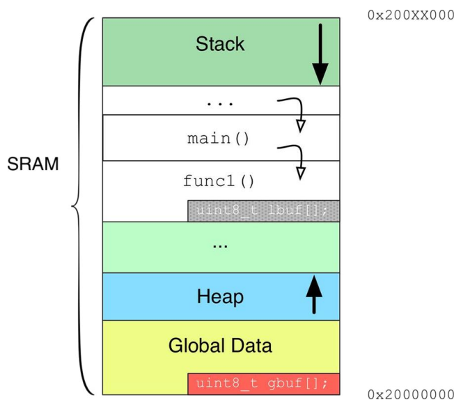
Figure 9: The difference between a variable allocated locally and globally
