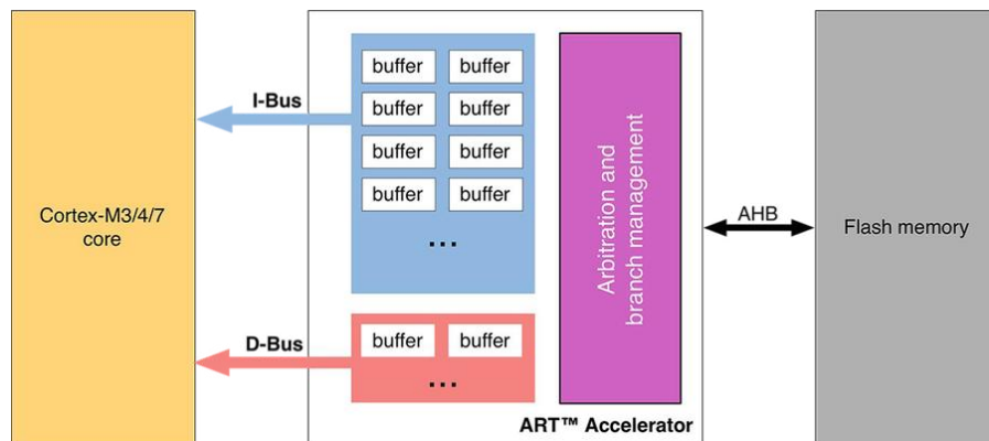
Figure 2: The main blocks forming the ART™ Accelerator
