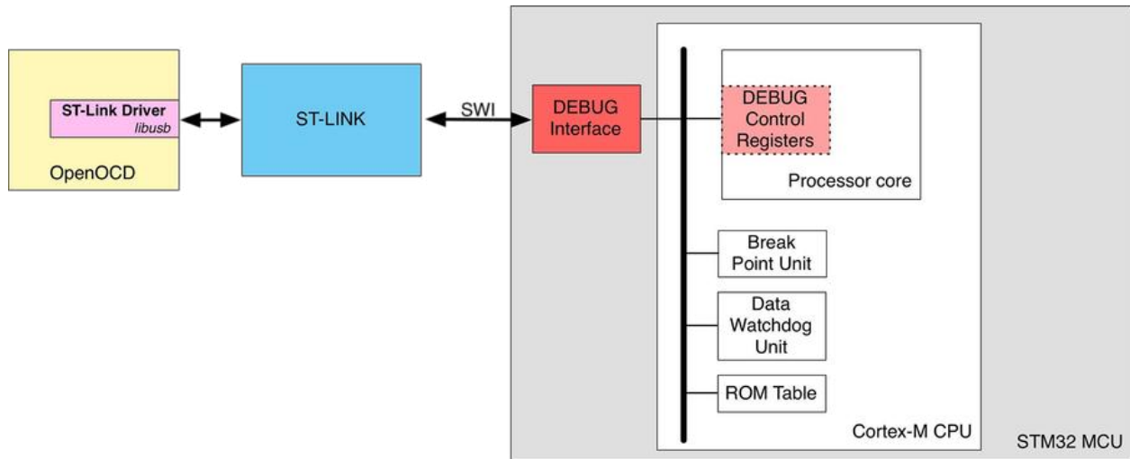
Figure 20: Debug components in Cortex-M microcontrollers
