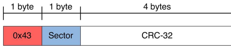
Figure 5: The structure of the CMD_ERASE
