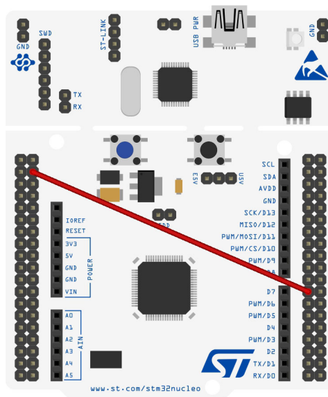
Figure 4: How to route the MCO pin to the TIM3_ETR pin in a Nucleo-F030R8 board
