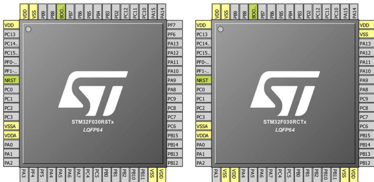
Figure 7: The STM32F030RC MCU requires four additional power sources compared to the STM32F030R8 one
