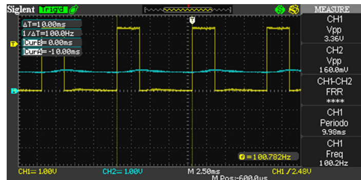
Figure 26: The effect of a low-pass filter with cut-off frequency equal to 3.7Hz
