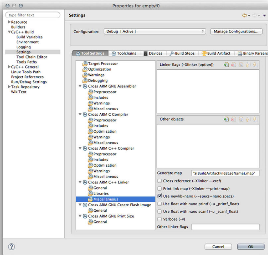
Figure 10: How to select newlib/newlib-nano run-time library
