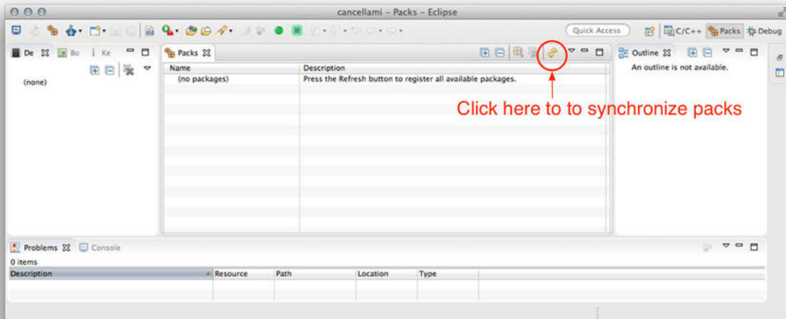
Figure 14: How synchronize Eclipse with the Keil Packs repository
