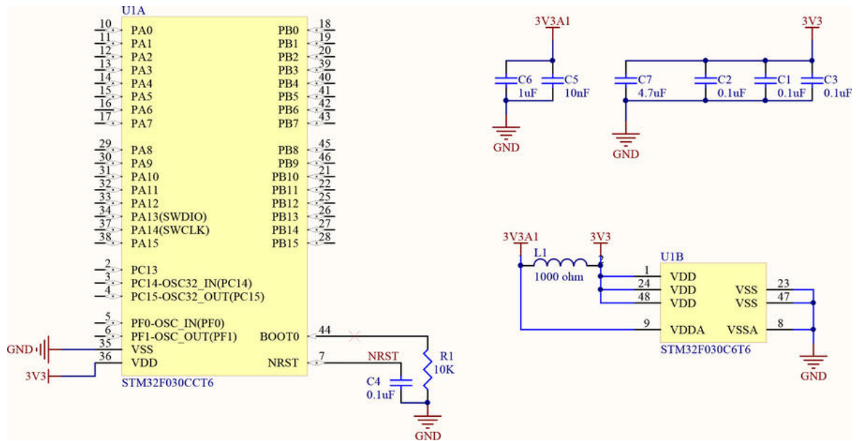
Figure 2: The minimal reference schematics for an STM32F030 MCU
