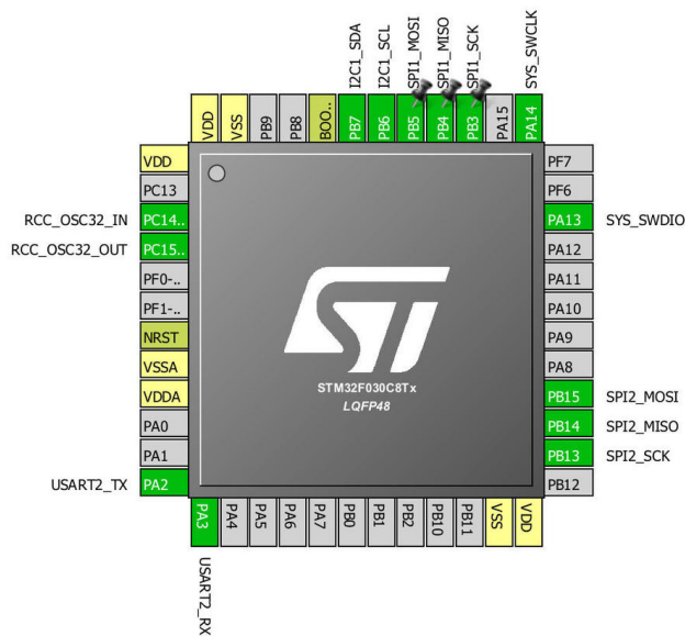
Figure 10: Pre-visualizing the MCU can help you during board layout
