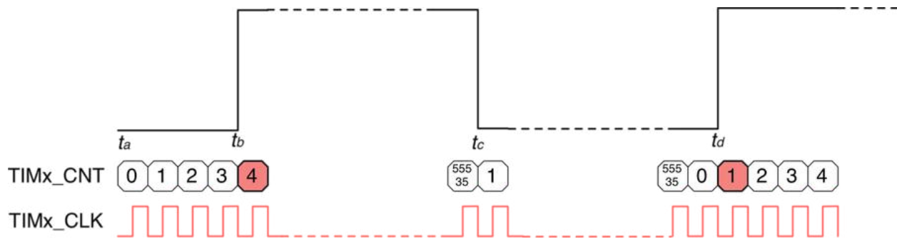
Figure 18: If the timer runs faster than the sample signal, then it overflows before the two rising edges are detected
