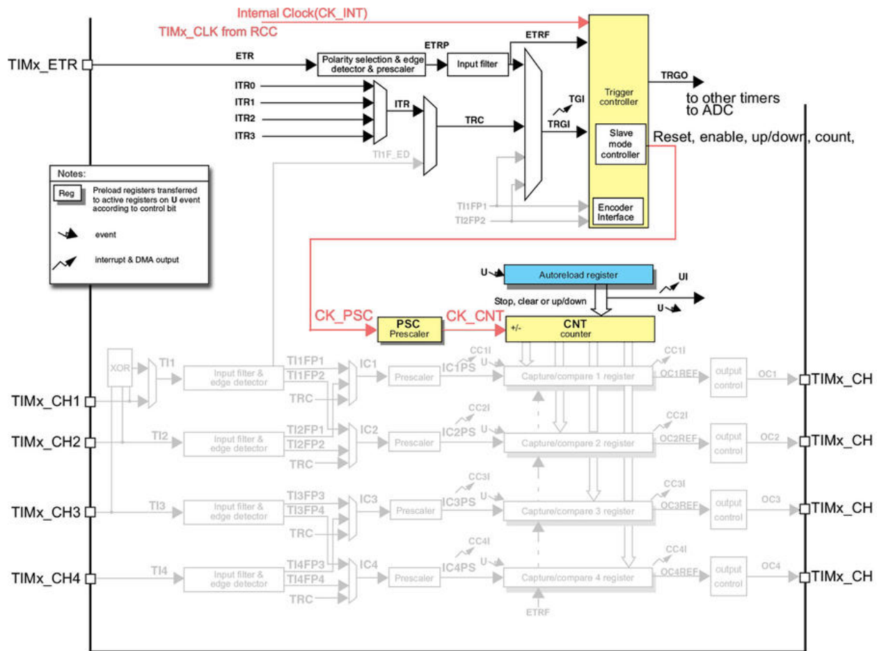
Figure 3: The structure of a general purpose timer
