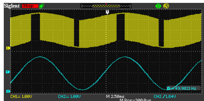
Figure 29: How timers allow to approximate a 50Hz sine wave using PWM
