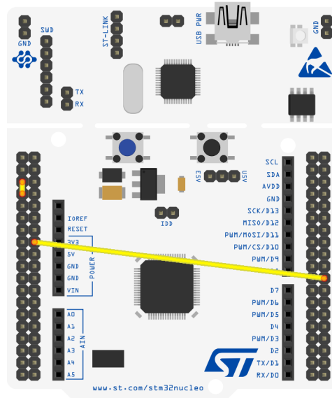
Figure 3: How to tie BOOT0 and BOOT1 pins to VDD in a Nucleo board so that MCU boots from SRAM
