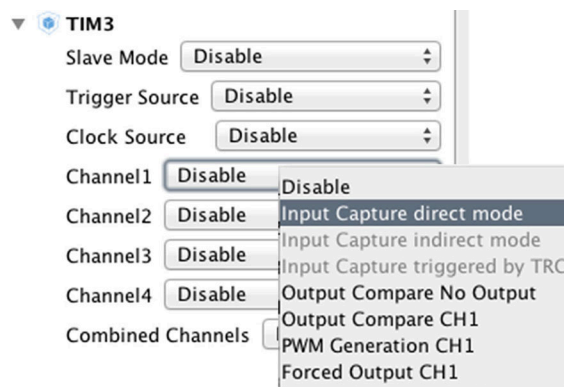
Figure 19: How to enable a channel in input capture mode
