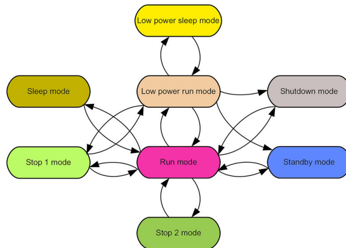
Figure 9: The allowable power mode transitions in an STM32L4 MCU
