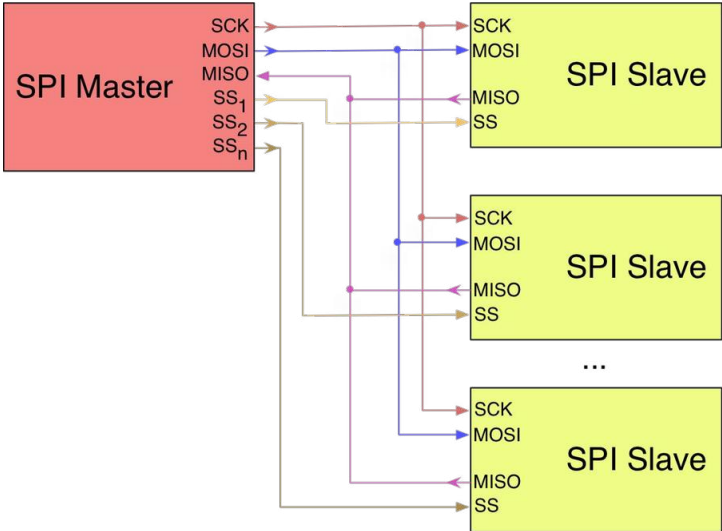
Figure 1: The structure of a typical SPI bus
