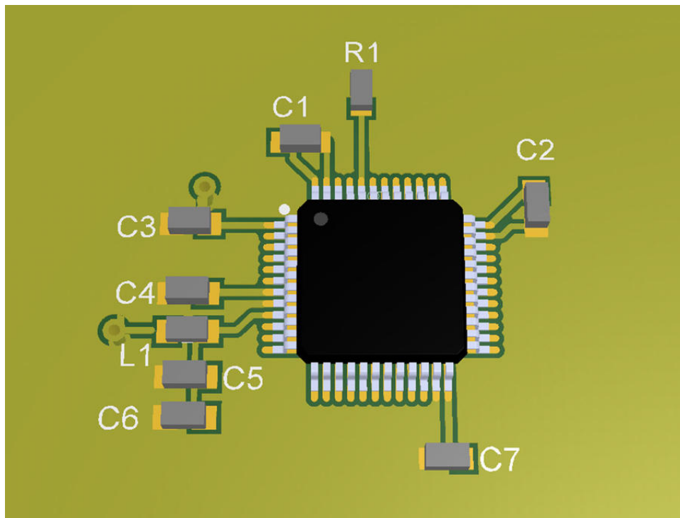
Figure 3: The preferred way by the author of this book to place decoupling capacitors
