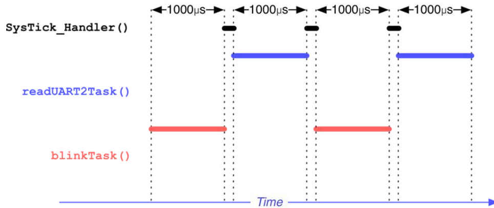
Figure 3: The impact of the context switch on tasks scheduling
