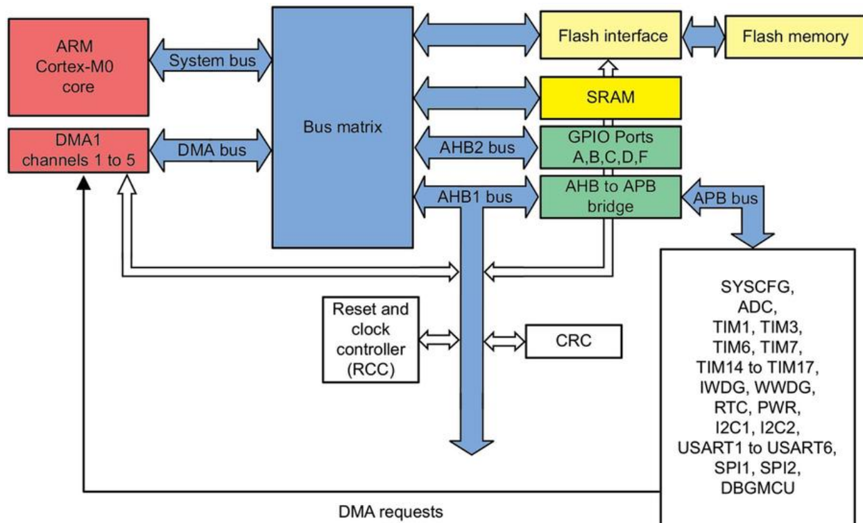
Figure 1: Bus architecture of an STM32F030 microcontroller
