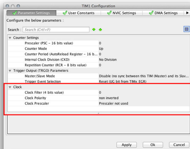
Figure 7: How to configure a timer working in ETR2 mode
