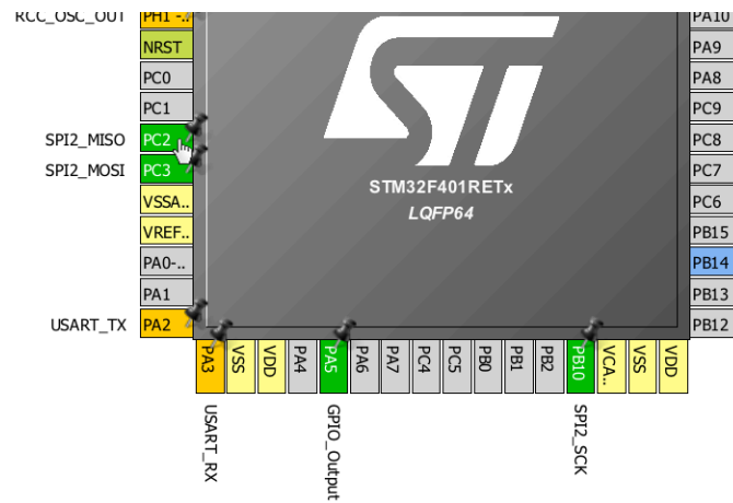
Figure 6: Alternate mapping of peripherals
