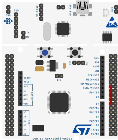
Figure 5: How to route the MCO pin to the TI2FP2 pin in a Nucleo-F030R8 board
