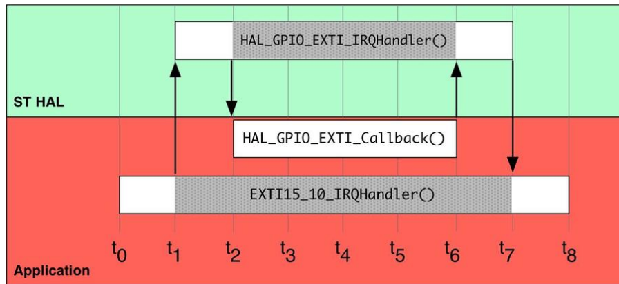
Figure 4: How an IRQ is processed by the HAL
