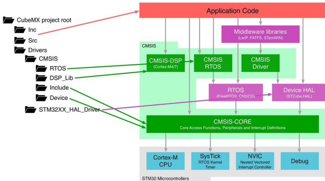
Figure 13: The generated code compared to the CMSIS architectural view
