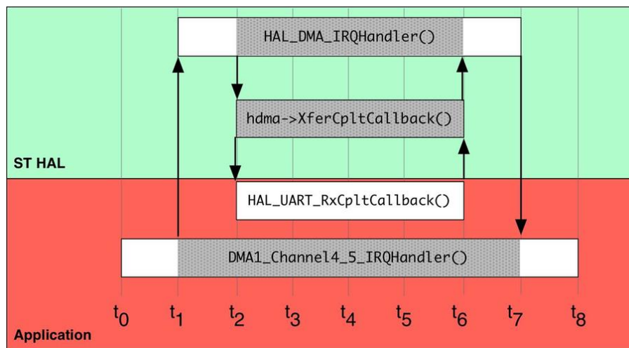
Figure 7: The call sequence generated by the HAL_DMA_IRQHandler()
