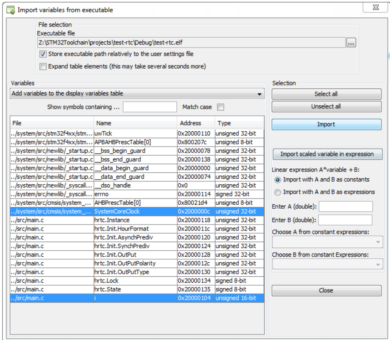
Figure 23: How to import variables inside STM Studio
