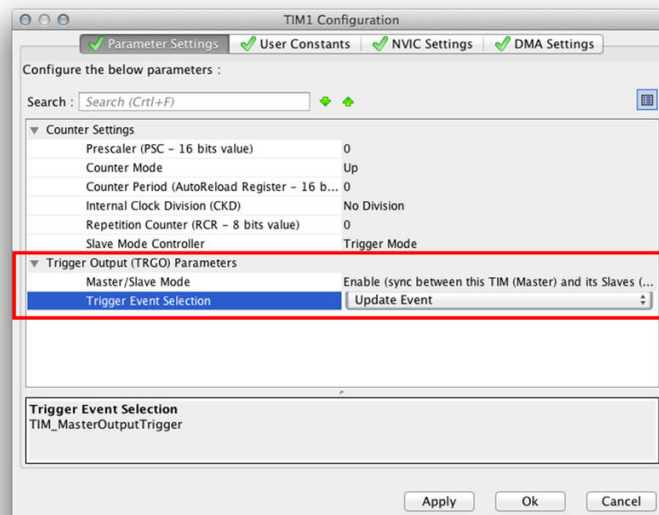
Figure 14: How to configure a timer in master mode
