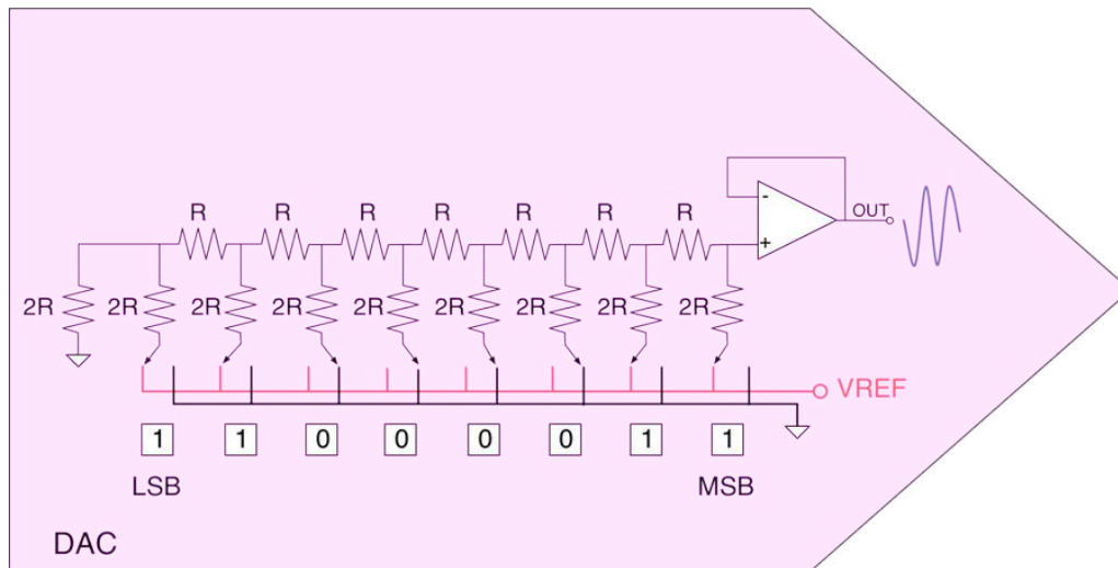
Figure 2: How a R-2R network can be used to convert a digital quantity to an analog signal
